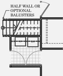
STAIRS TO OPTIONAL BONUS ROOM & LAUNDRY ROOM CONFIGURATION
